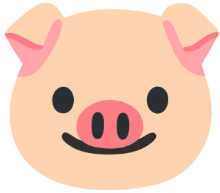
pig
