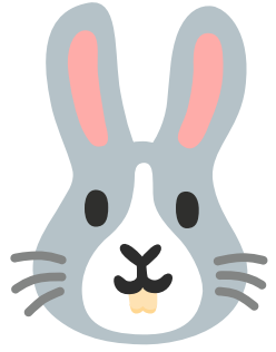
bunny
