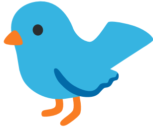
bird
